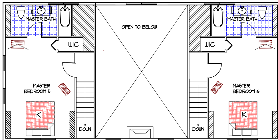
CABIN 5 SECOND FLOOR
