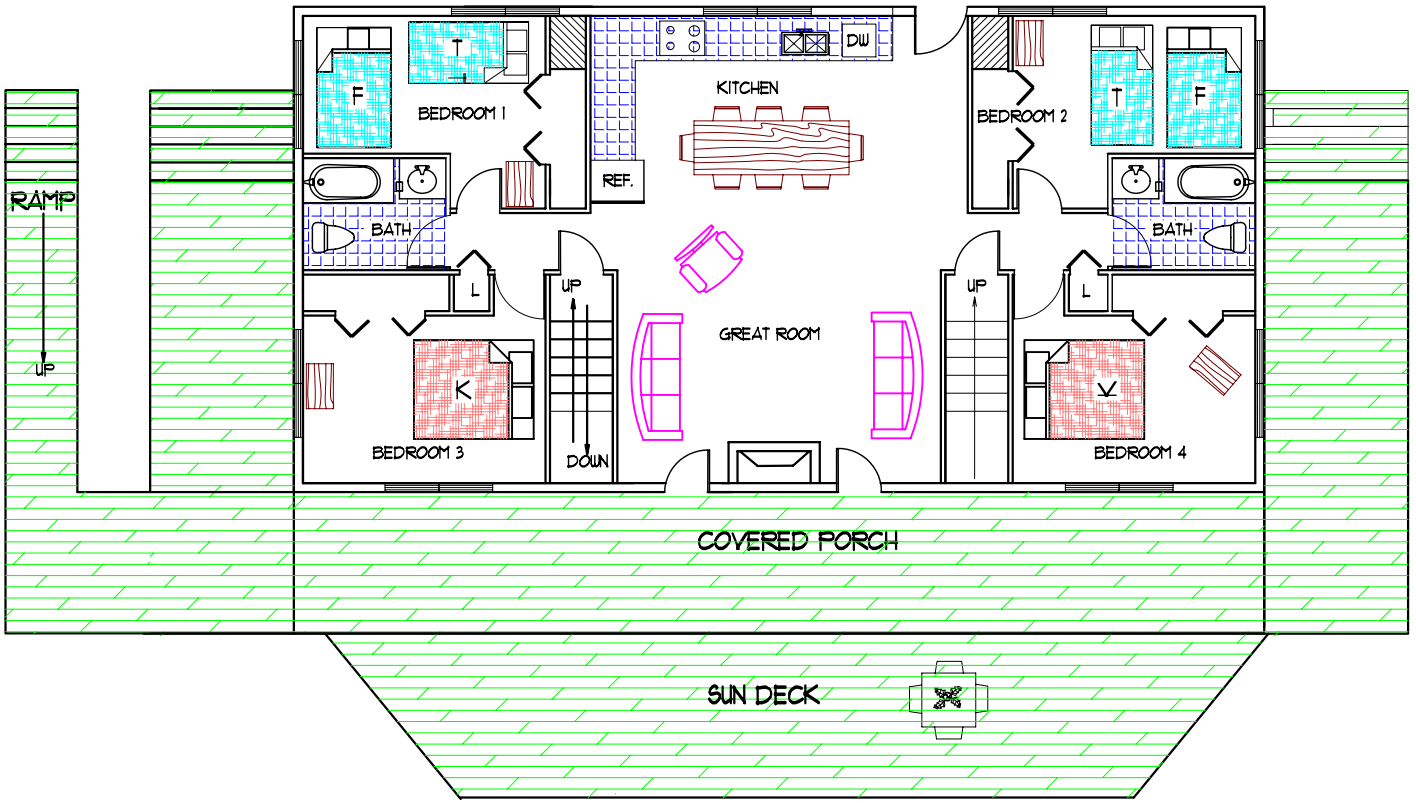
CABIN 5 FIRST FLOOR
